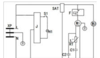
SD-206/336/416AELC/AEL
