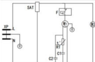
SD-206/336/416AEC/AE
