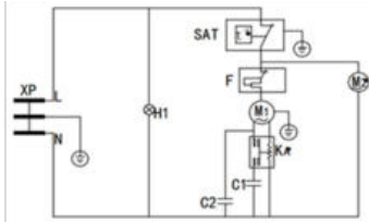
SD-516AMC/AM
