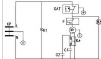
SD-516AMC/AM
