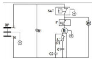
SD-206/336/416 AMC/AM
