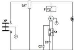
SD-516AEC/AE
