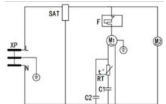
SD-206/336/416AEC/AE
