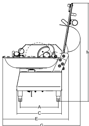
Standard 1 Mozzo a 3 lame Hub 3 blades
