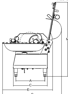
Standard 1 Mozzo a 3 lame Hub 3 blades
